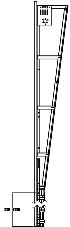
VERTICAL LIFT TRACK DETAIL (OPTIONAL)
