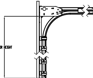
LOW HEADROOM TRACK DETAIL (OPTIONAL)
