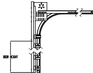
STANDARD LIFT TRACK DETAIL (OPTIONAL)
