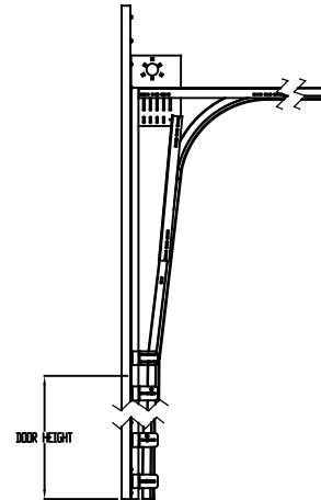
HIGH LIFT TRACK DETAIL (OPTIONAL)
